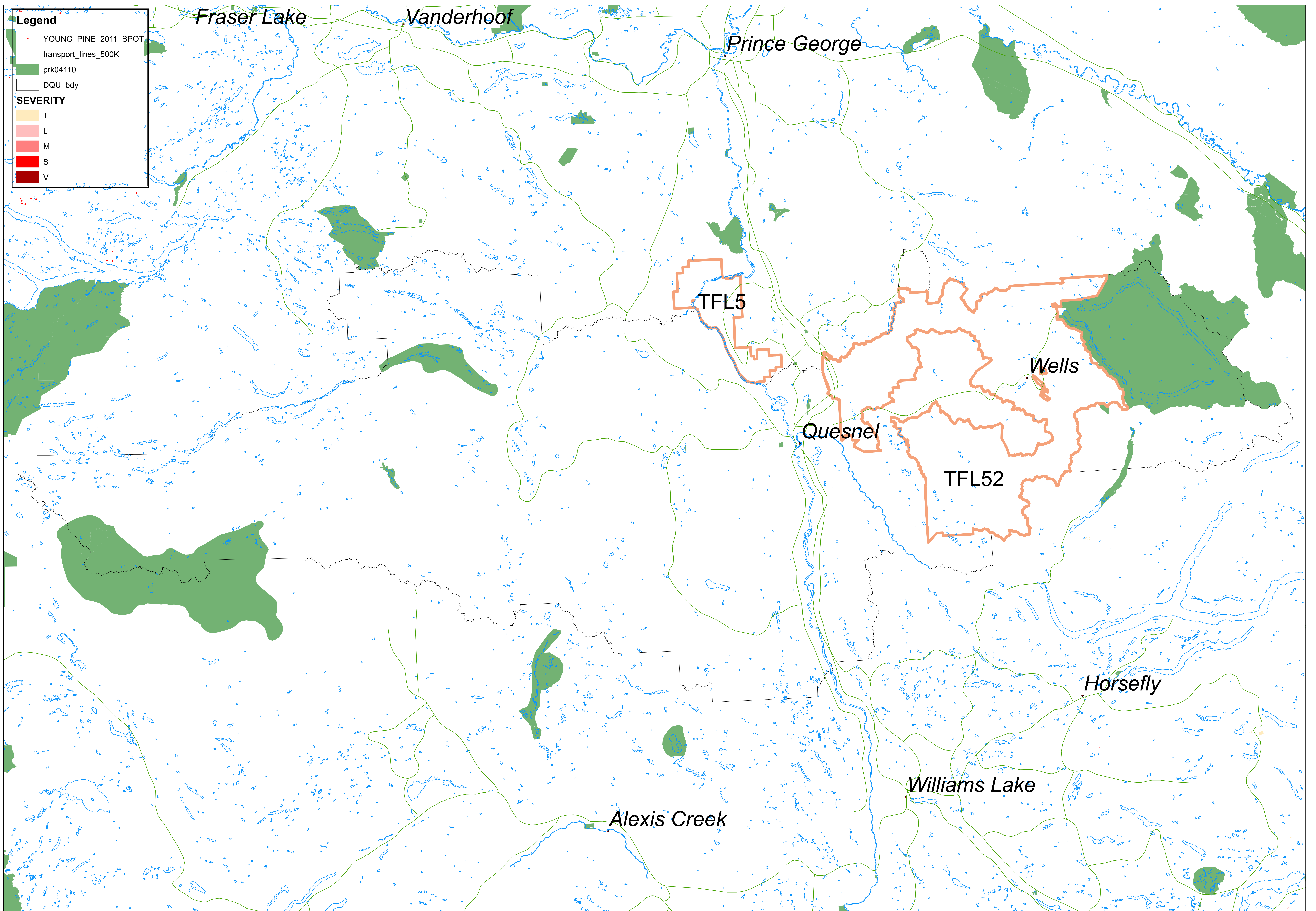
2011 Young Pine Mortality in Quesnel TSA
